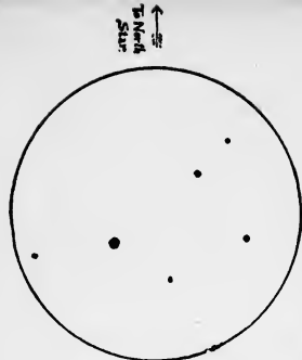
The Pleiades as seen by Ordinary Eyes
